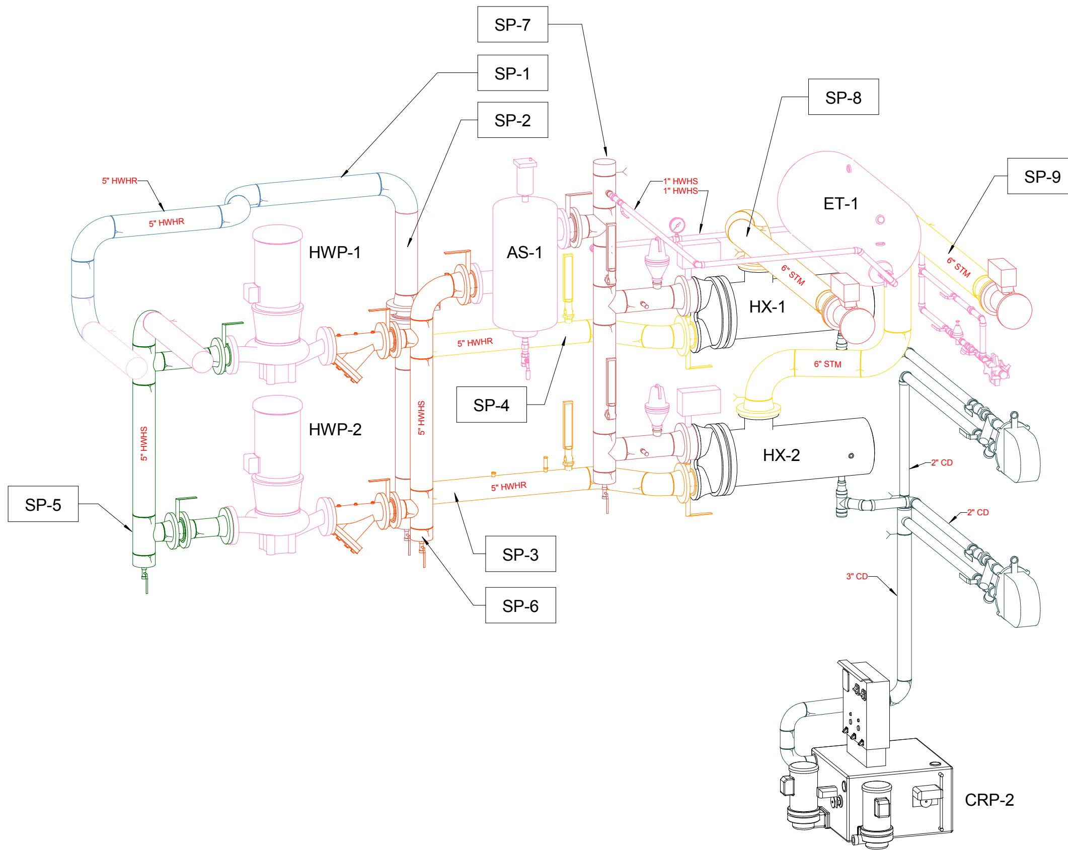
Boiler Room Spool Map
